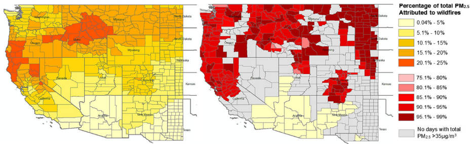
Fig. 1 Fraction of PM_{2.5} attributable to wildfires by county during fire seasons (May–October) in the present day (2004–2009), on all days (left panel), and on the subset of days that had total PM_{2.5} > 35 \mu\text{g}/\text{m}^3 (The National Ambient Air Quality Standards (NAAQS) threshold; right panel)
