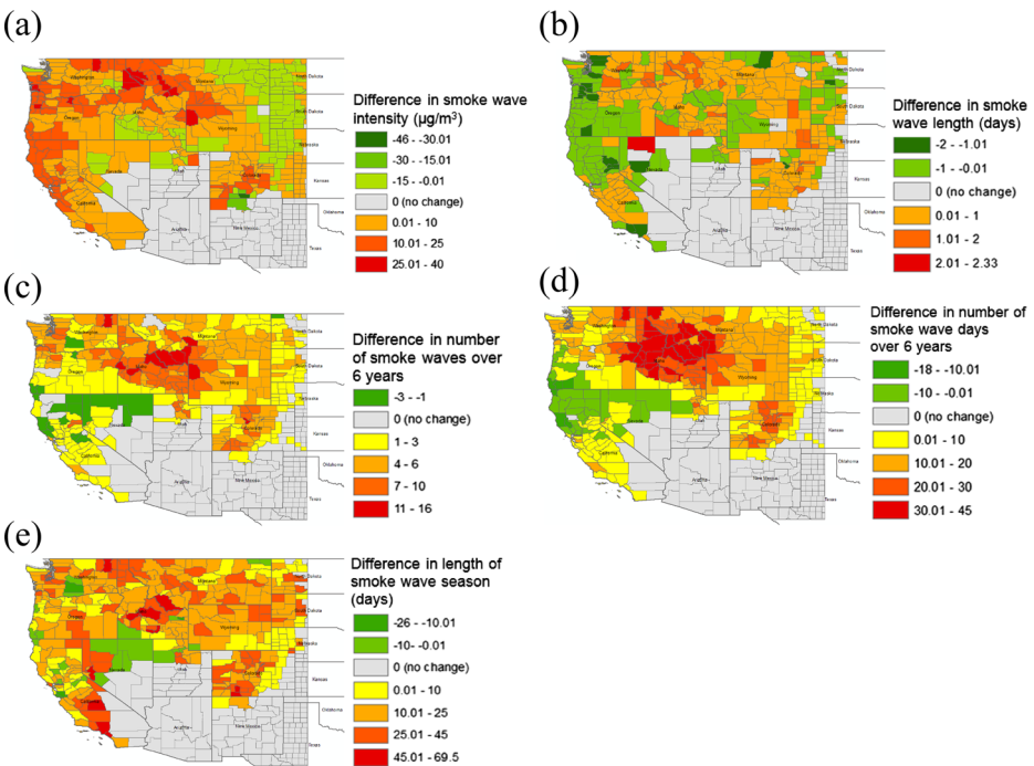
Fig. 2 Difference in smoke wave characteristics in the future (2046–2051) under climate change and in the present day (2004–2009) during fire seasons (May–October). Positive changes (in warm colors) indicate increases under climate change, while negative changes (in cool colors) indicate decreases under climate change. Panels show (a) average intensity of smoke waves; (b) average length of smoke waves; (c) total number of smoke waves during a 6-year period; (d) total number of smoke wave days during the 6-year period; and (e) average length of the smoke wave season
